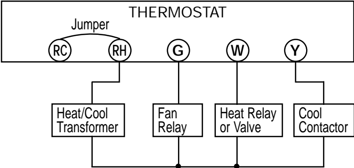
4-wire Heat/Cool System
