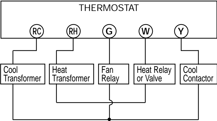
5-wire Heat/Cool System
