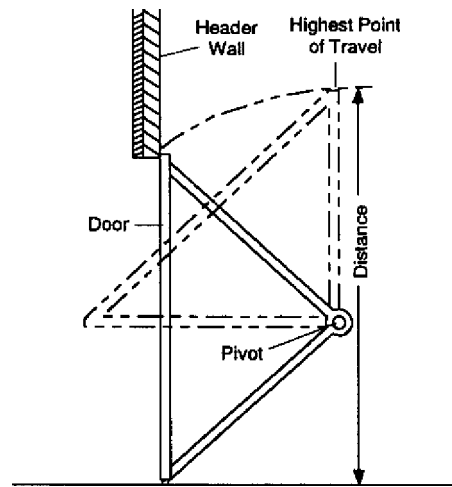
One-piece door without track pivot hardware
