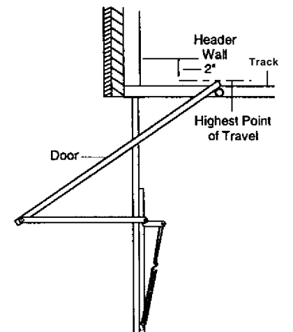
One-piece door with horizontal track
