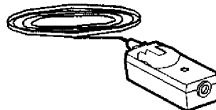
(2) Safety Reversing Sensors (1 Sending Eye and 1 Receiving Eye) with 2-Conductor White & White/Black Bell Wire attached
