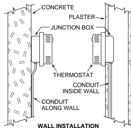
WALL INSTALLATION The mounting plate for this thermostat has two holes 3/16" apart for attaching the control on a standard switch box.
