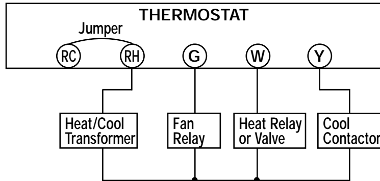
4-wire Heat/Cool System
